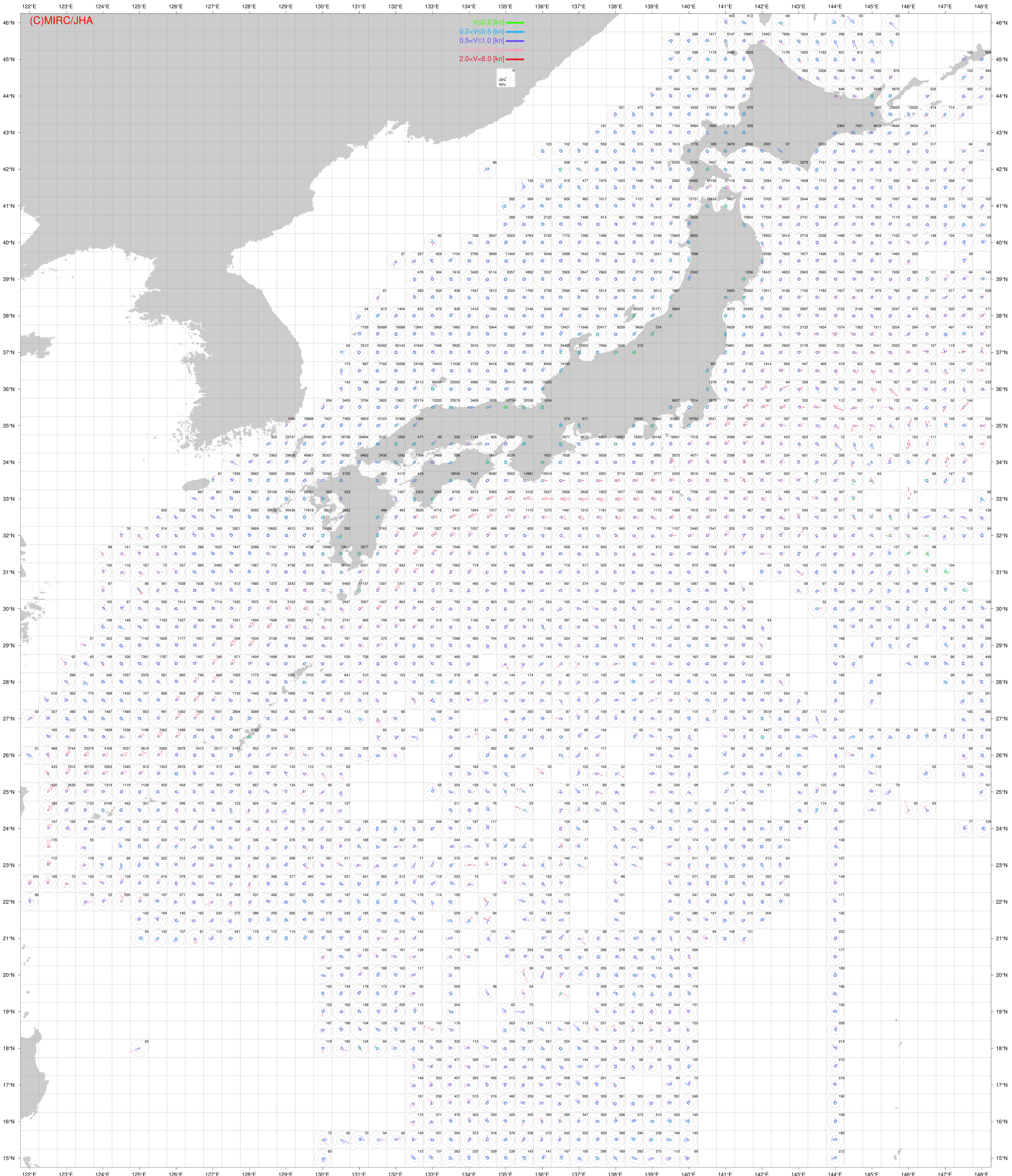
ADCP Current Histogram in 16 directions in 30' square (N≥50) at 10 m depth in Jan.1986-Dec.2001
